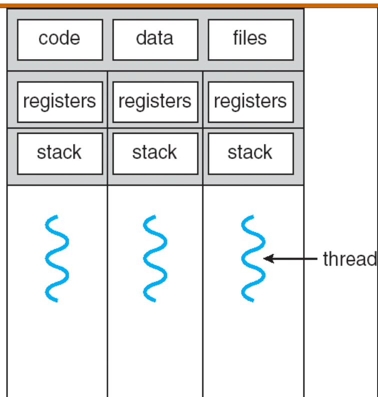
multithreaded process
