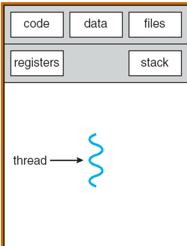
single-threaded process
