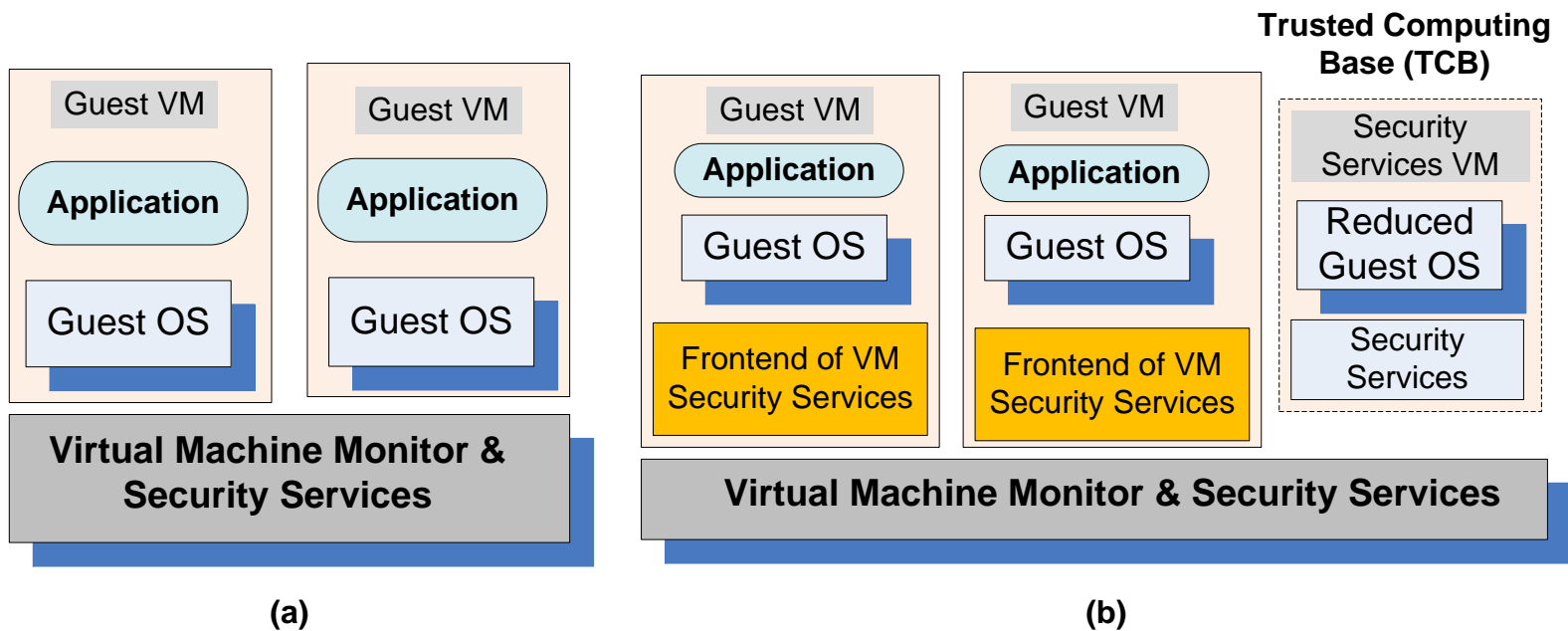
(a) Virtual security services provided by the VMM; (b) A dedicated security VM.
